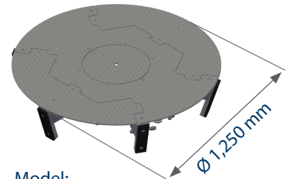
Model: Two-piece platform Useable volume: up to approx. 3,000 liters Weight: 26 kg
